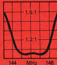
VSWR CURVE
